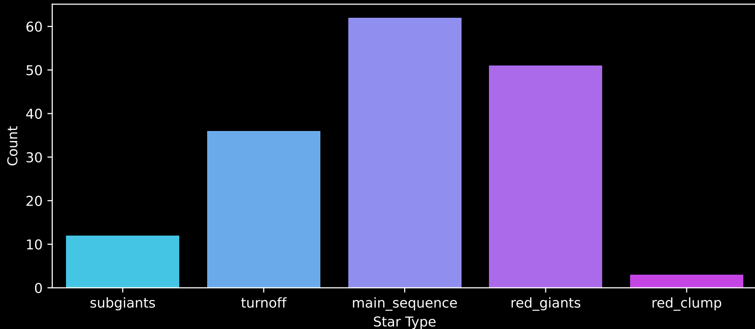
APOGEE DR17 Field: [280-22-O_TESS] Count plot of Star Type
