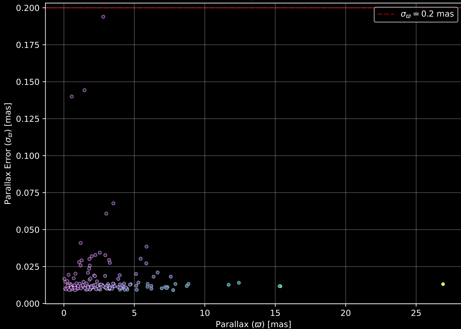
APOGEE DR17 Field: [280-22-O_TESS] Parallax Quality (n= 164)
