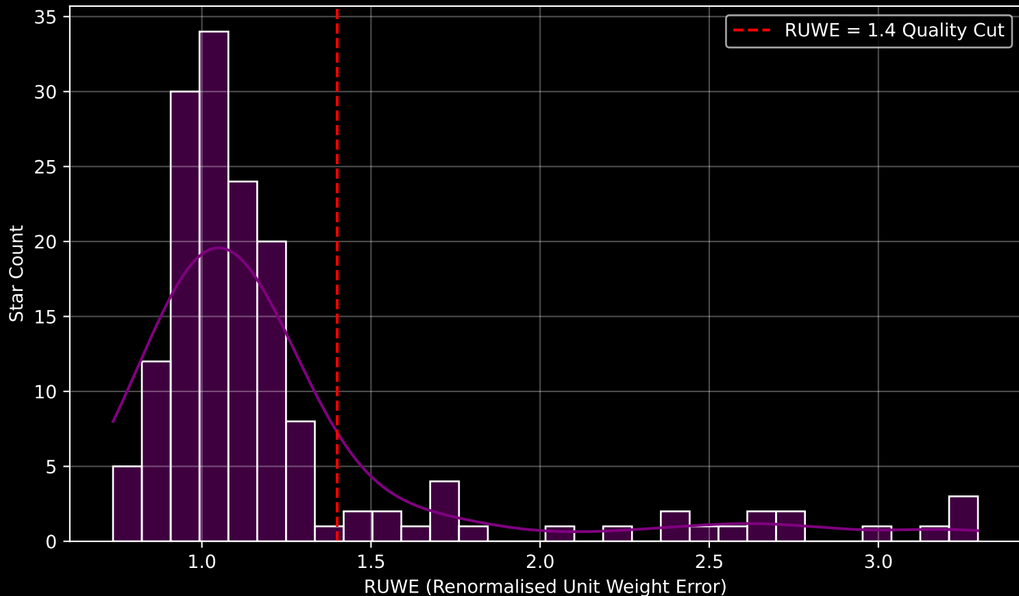
GAPOGEE DR17 Field [280-22-O_TESS] RUWE Distribution (n= 159)
