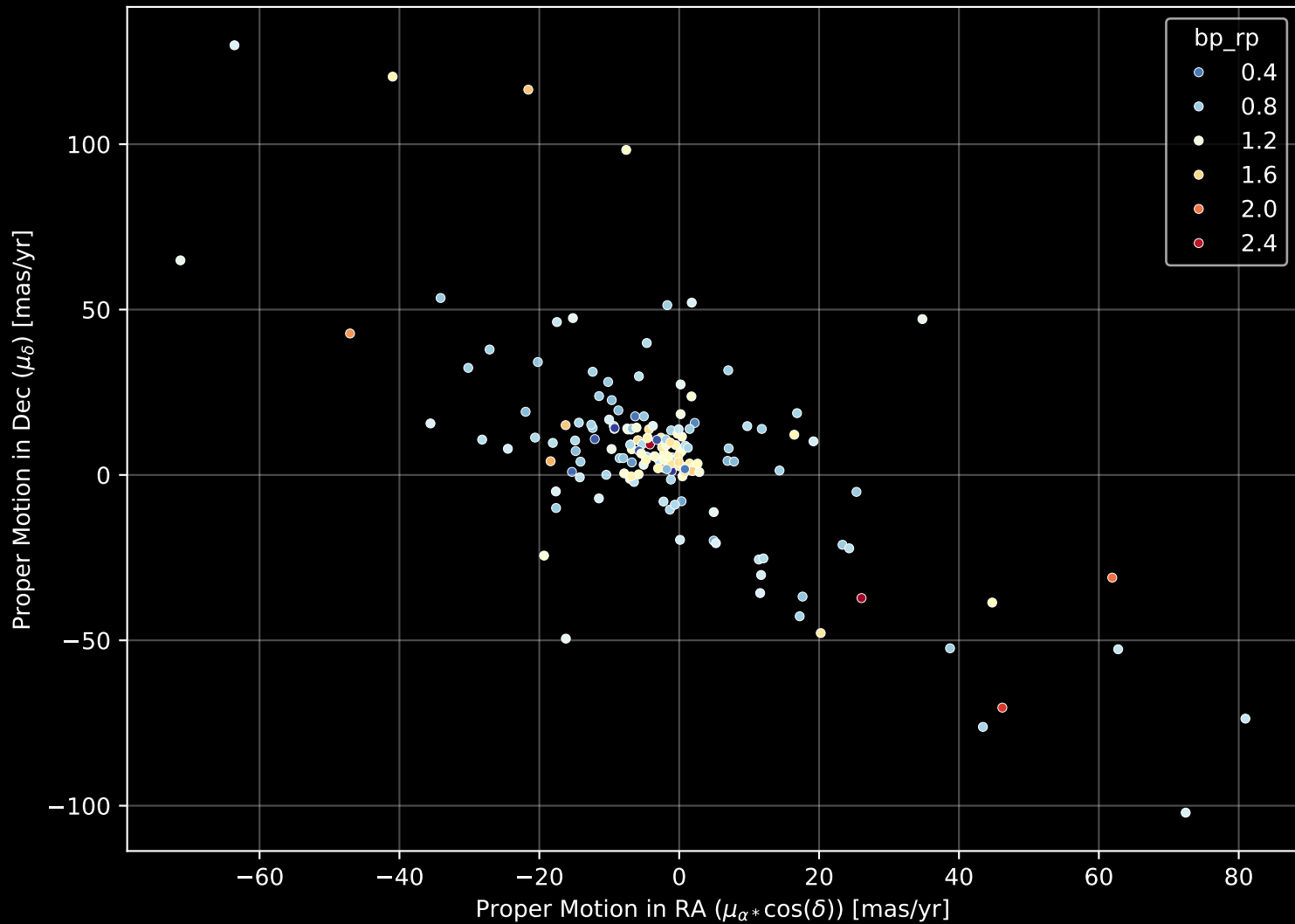
APOGEE DR17 Field: [280-22-O_TESS] Proper Motion Diagram (n= 164)
